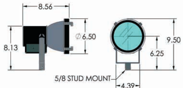
200W HMI SUPER-SUN GUN (SSG-200) DIMENSIONS
