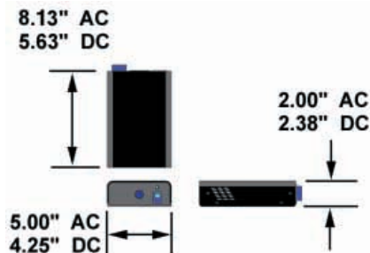
200W HMI AC AND DC BALLAST DIMENSIONS
