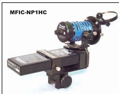
Dimmer Mini Fill with self contained NP1 holder with optional FNP1S battery and dichroic filter (MFDF)
